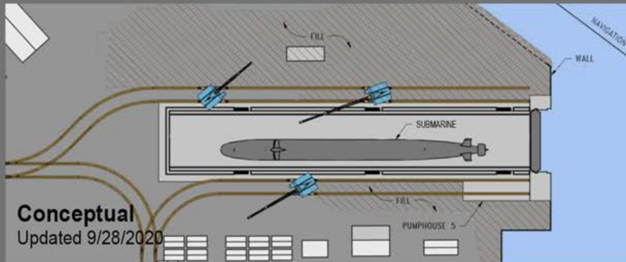
Uncovered Dry Dock replacement with Portal Cranes
